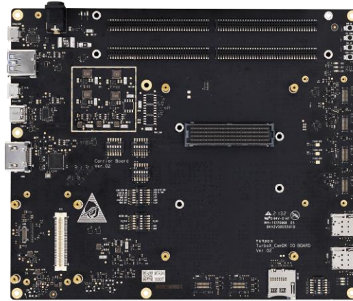
Main IO Board
