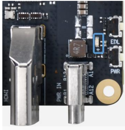
Figure 2-3. Power Indicator
