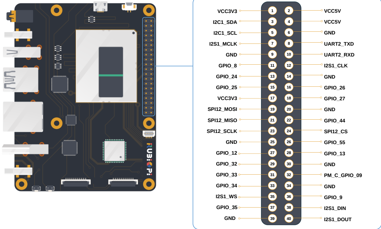
Figure 3-1. Default Functions of the 40-pin Connector Pins
