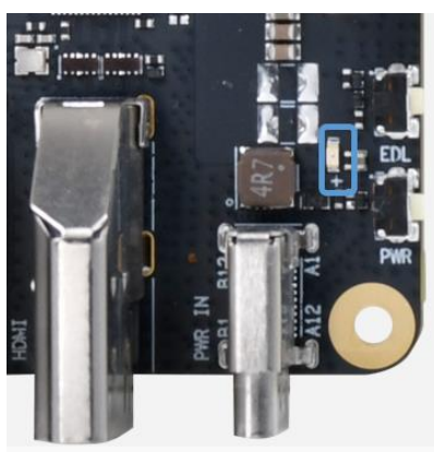
Figure 2-3. Power Indicator
